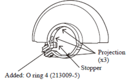
Wheel cover 125AK assembly (123099-9)
