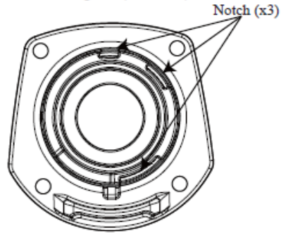
Bearing box (319462-4)
