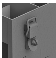
2 padlockable latches to secure the cover (padlock not included)
